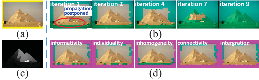
Figure 5. Visualization of the designed propagation process. (a) shows the input image with boundary seeds (yellow). (b) displays the propagations in several key iterations, and the expansions of labeled set \mathcal{L} are highlighted with light green masks. (c) is the final saliency map. The curriculum superpixels of the 2nd iteration decided by informativity, individuality, inhomogeneity, connectivity, and the final integrated result are visualized in (d), in which the magenta patches represent the learned superpixels in the 1st propagation, and the regions for the 2nd diffusion are annotated with light green.
