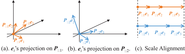
Figure 2: Illustration of scale alignment. The lengths of projected e_i ( i = 1, 2, \dots, d ) by different projection matrices are summed up to the same value. Here d is simply set to 3 for visualization.
