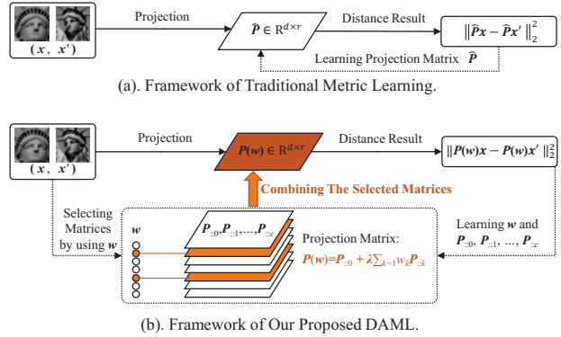
Figure 1: The comparison of traditional metric learning and our proposed model. (a) The traditional method learns a single global projection matrix \widehat{P} to distinguish the similarity of (x, x') . (b) Our proposed DAML jointly learns multiple projection matrices P_{:,0}, P_{:,1}, \dots, P_{:,c} and their weight vector w \in \mathbb{R}^c for each data pair (x, x') .
